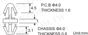
P.C.B Φ4.0 THICKNESS 1.6 CHASSIS Φ4.0 THICKNESS 0.8 Unit:mm
