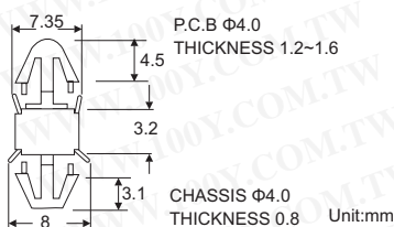
P.C.B Φ4.0 THICKNESS 1.2~1.6 CHASSIS Φ4.0 THICKNESS 0.8 Unit:mm
