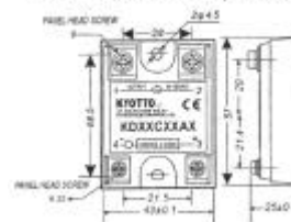
OUTLINE DIMENSIONS (unit:mm)
