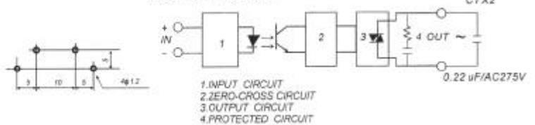
EQUIVALENT CIRCUIT
