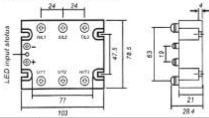
OUTLINE DIMENSIONS (unit:mm)
