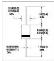
DO-41
