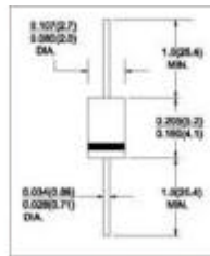
DO-15
