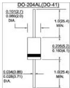
DO-41
