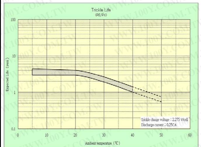
4. 浮充壽命 (Trickle Life)
