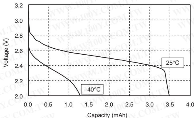
MS621T Discharge Characteristics
