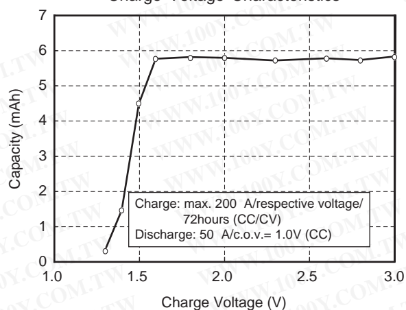
Charge Voltage Characteristics
