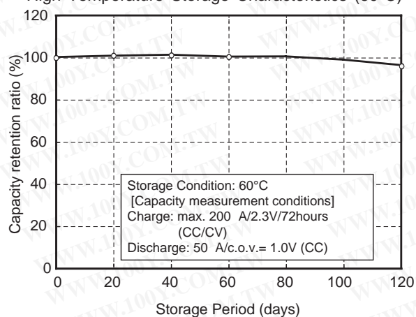
High Temperature Storage Characteristics (60°C)
