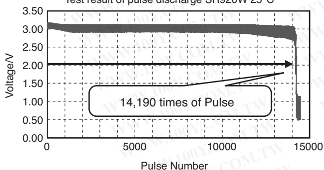
SR920W (2 pcs in series)
