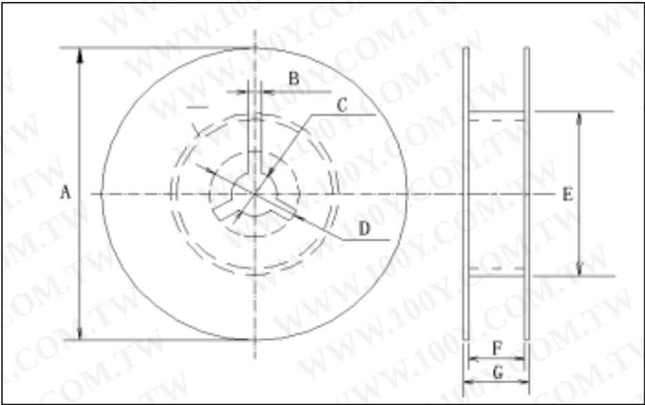
卷盘尺寸 Reel Dimensions (unit: mm)
