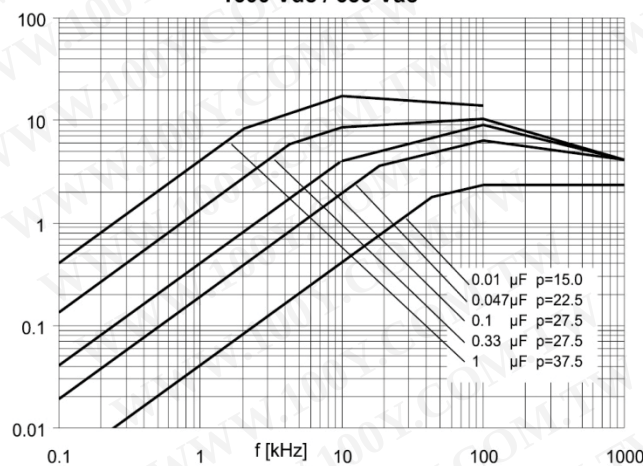
1600 Vdc / 650 Vac
