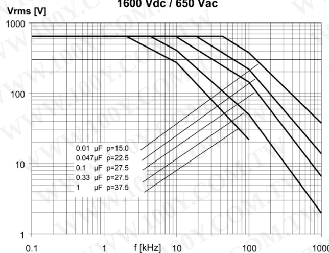
1600 Vdc / 650 Vac
