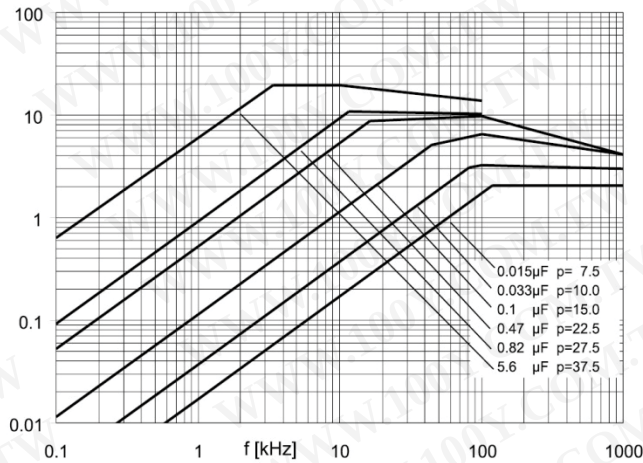
250 Vdc / 180 Vac
