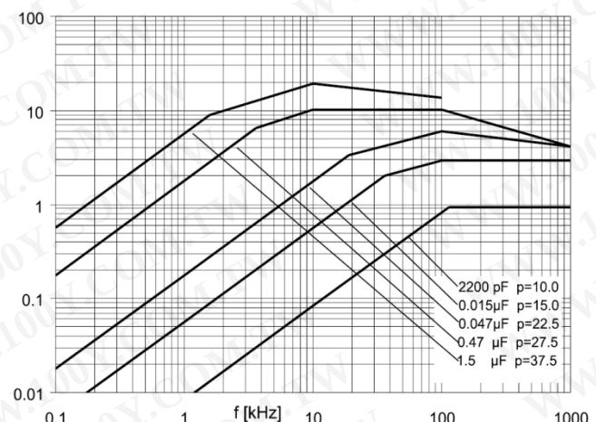
1000 Vdc / 600 Vac
