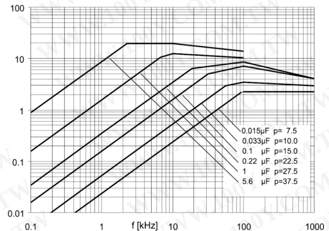
400 Vdc / 250 Vac
