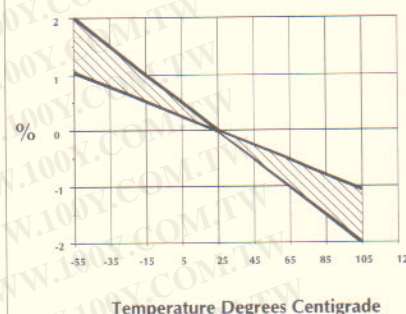
Dissipation Factor vs Temperature
