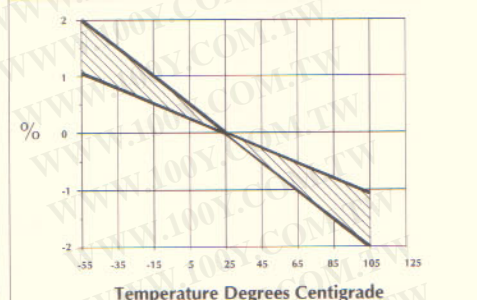
Figure 3 Dissipation Factor vs Temperature
