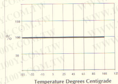
Figure 4 Voltage Derating vs Temperature
