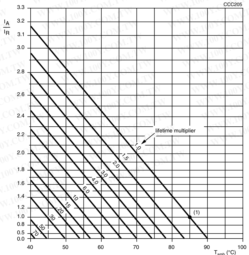
Fig.6 Multiplier of useful life as a function of ambient temperature and ripple current load
