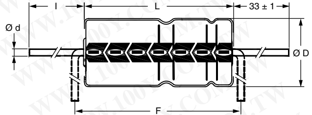
Form AA: Axial in box Case Ø D x L = 10 mm x 30 mm to 21 mm x 38 mm
