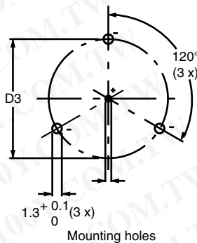
Form MR: Case Ø D x L = 15 mm x 30 mm to 21 mm x 38 mm Especially for applications with severe shocks and vibrations
