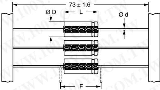
Form BR: Taped on reel Case Ø D x L = 6.5 mm x 18 mm to 15 mm x 30 mm Form BA: Taped in box (ammopack) Case Ø D x L = 6.5 mm x 18 mm to 10 mm x 25 mm
