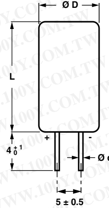
Case \text{Ø D} \times L = 8.2 \times 11 \text{ mm} only
