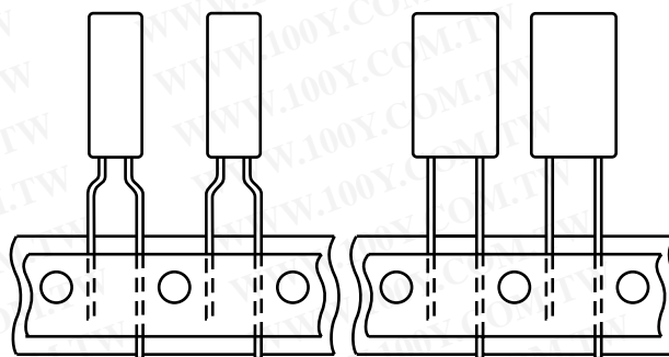
Case \text{Ø D} \times \text{L} = 5 \times 11 and 8.2 \times 11 mm Pitch F = 5 mm
