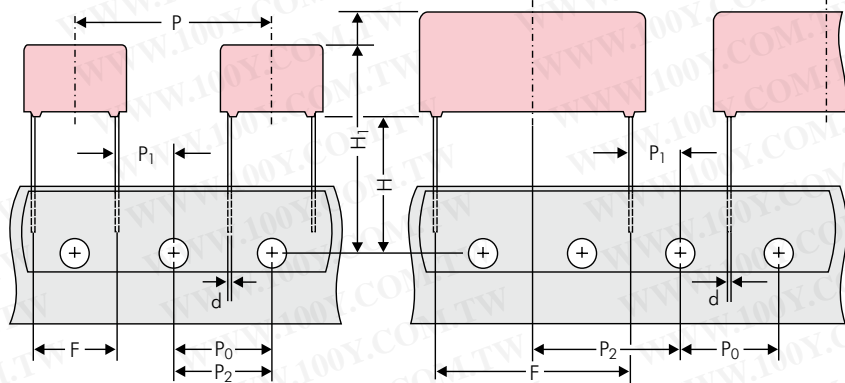
Diagram 2: PCM 10/15 mm
