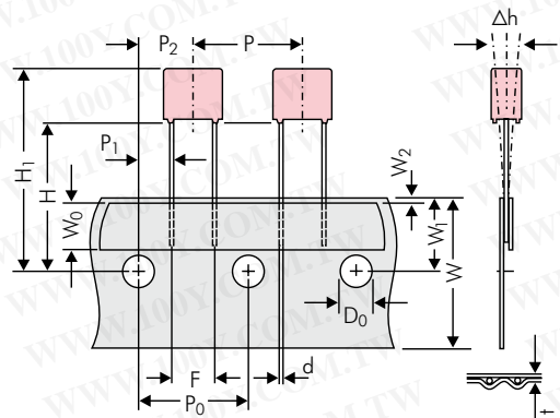
Diagram 1: PCM 2.5/5/7.5mm
