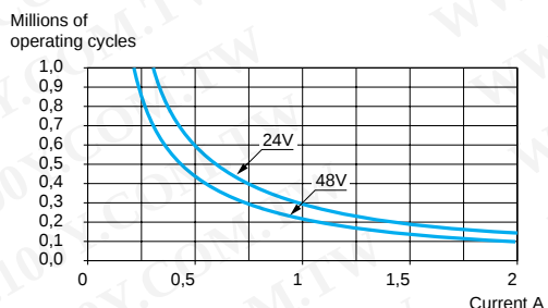
AC 15 curves (5)
