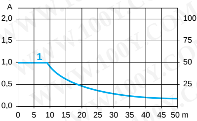
1 Cables ABF T2●●●●● c.s.a. 0.08 mm 2 (AWG 28)
