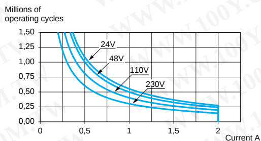
AC 15 curves (5)
