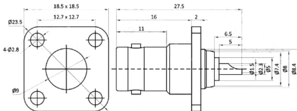
BNC Female Flange RF Connector Adapter
