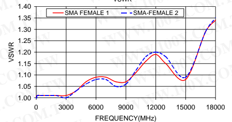
SF-SF50+ VSWR
