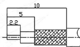
推荐剥线尺寸 Recommended stripping size
