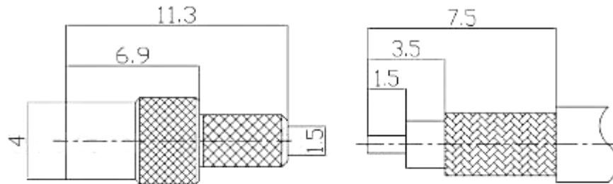
推荐剥线尺寸 Recommended stripping size
