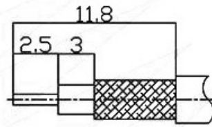
Recommended stripping size 推荐剥线尺寸
