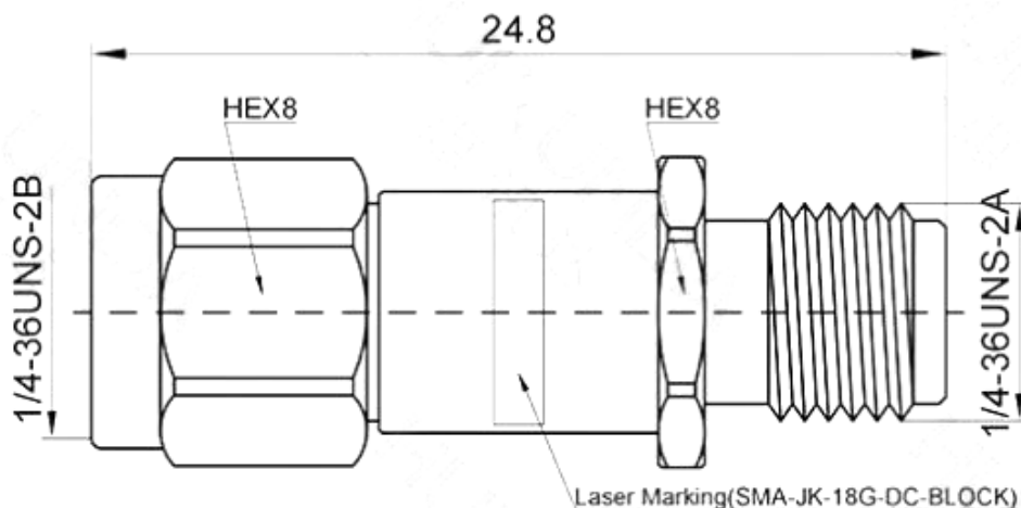
SMA Male To Female 2W 18G DC-BLOCK Connector
