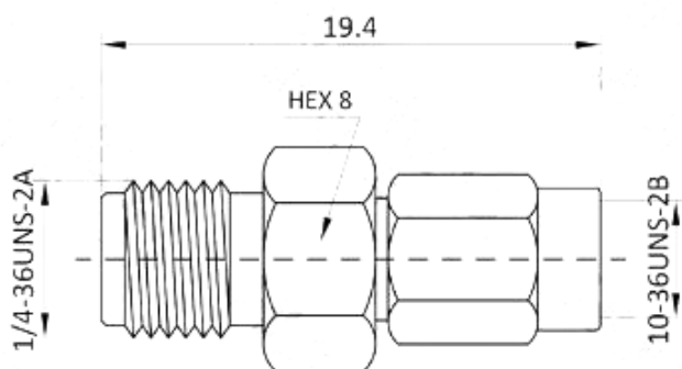
SMA Female to SSMA Male RF Connector Adapter
