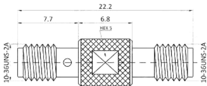
SSMA Female To Female Adaptor
