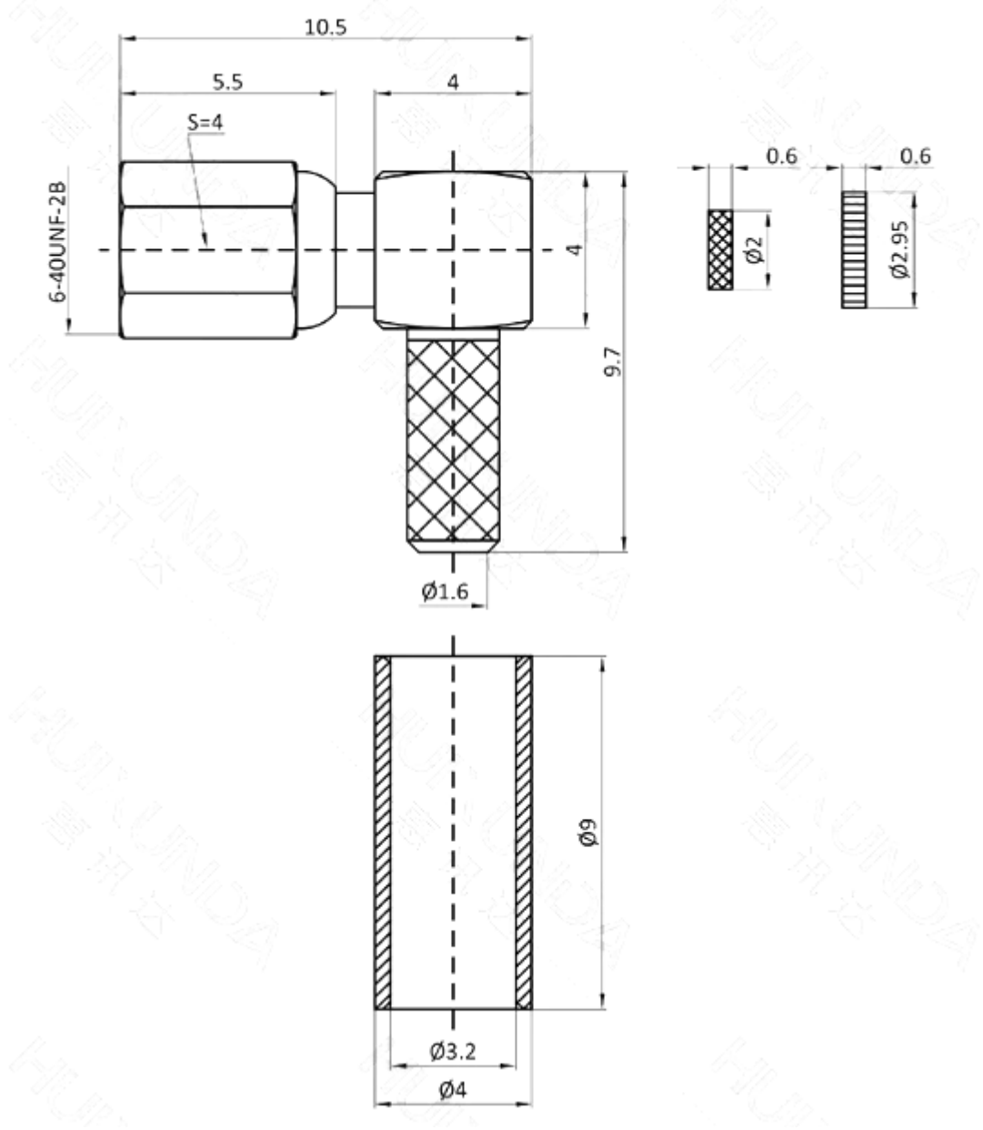
SSMC Female Right Angle Clamp Connector For RG316/50-1.5
