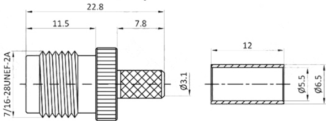
TNC Female Bulkhead Crimp Connector For 50-3/LMR200 Cable
