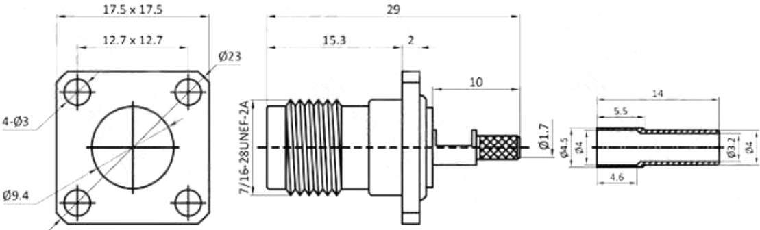
TNC Female Flange Crimp Connector For 50-1.5/RG316 Cable
