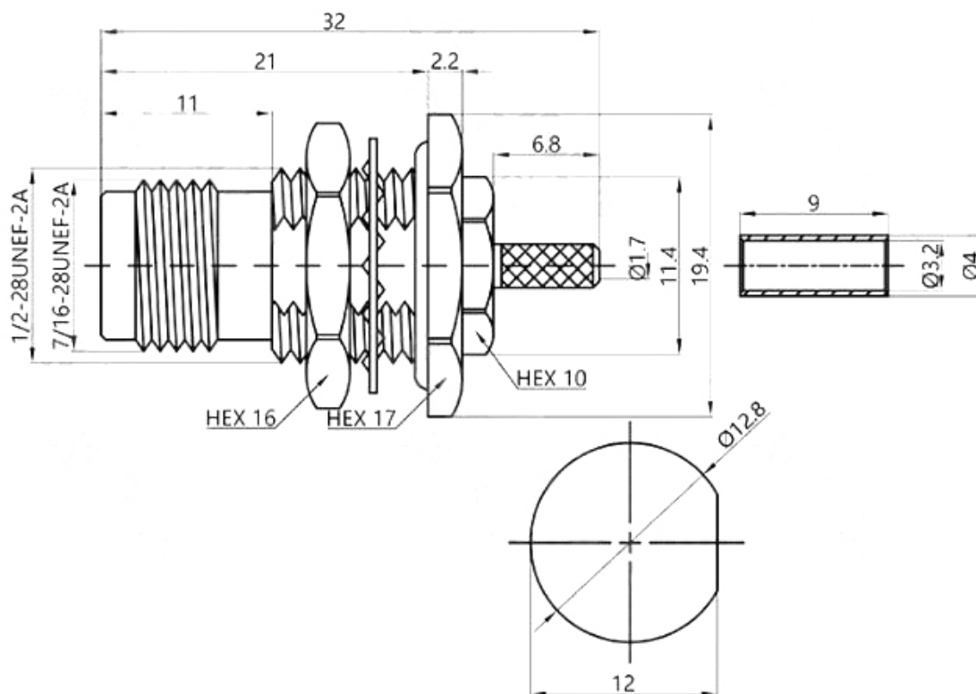
TNC Female Bulkhead Crimp Connector For 50-1.5/RG316 Cable
