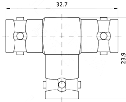
TRB/BNT Female to Female to Female TEE BN73 Adapter
