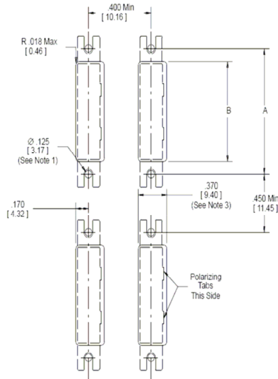
Rear Mount Panel Cutout
