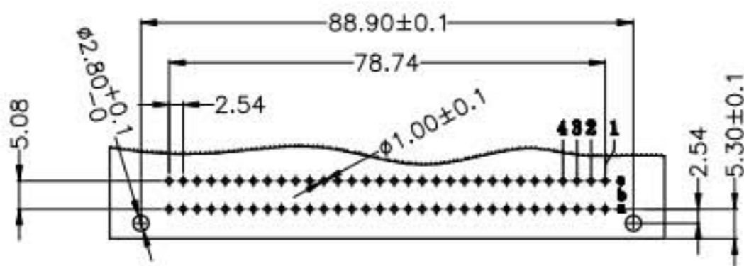
PCB LAYOUT(RECOMMENDED) (TOP VIEW TOL. :±0.05)
