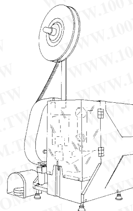
AMP-O-MATIC Side-Feed Stripper-Crimper III Machines 1320895-[] (409-10012)
