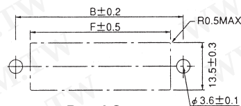
Panel Cutout
