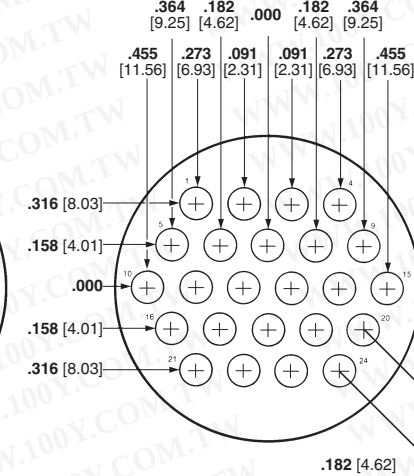
Arrangement 23-24 Max. Wire Ins. Dia. = .150 [3.81]
