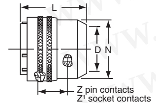
"CP" Potting Boot
