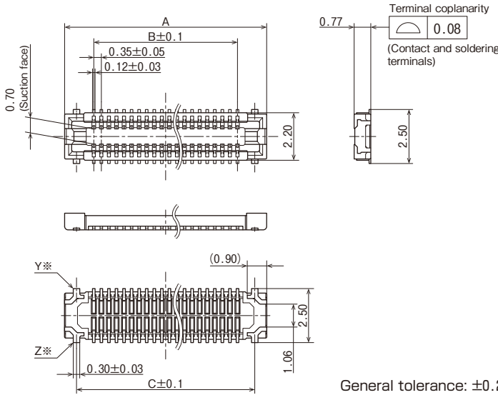
Dimension table
