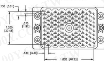
120 PIN PLUG
