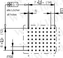
Board hole pattern (Component mounting side)
