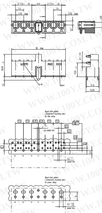
Dimensional drawings and board hole pattern
