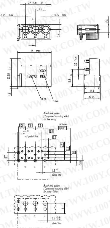
Dimensional drawings and board hole pattern
