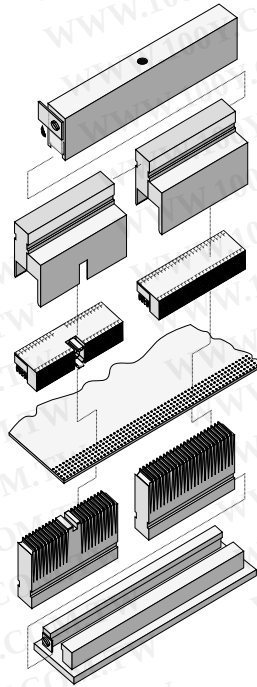
Modular press-fit tool for female connector modules 5+2
