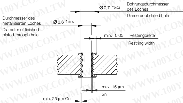
Metal Plating of Plated Through Hole
