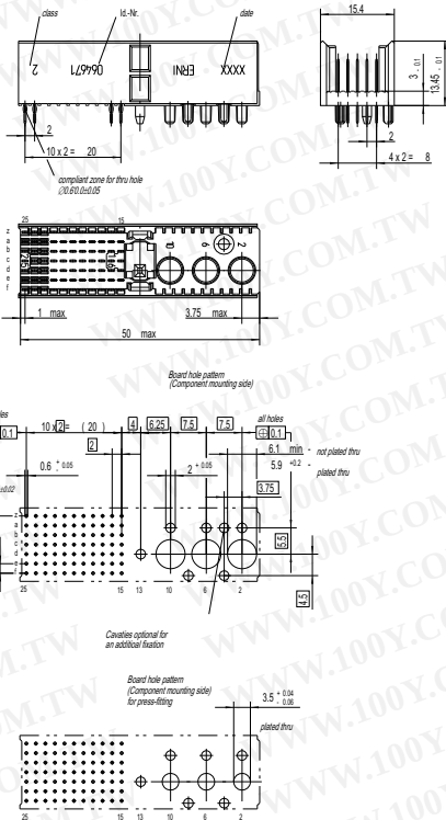
Dimensional drawings and board hole pattern
