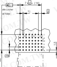
Board hole pattern (Component mounting side)
