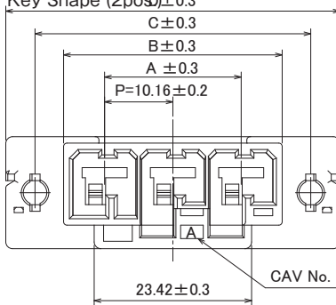
Another Key Shape (2pos.) ±0.3
