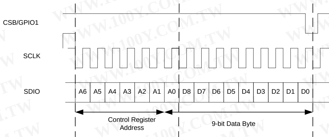
Figure 12: Register write operation using a 16-bit SPI Interface
