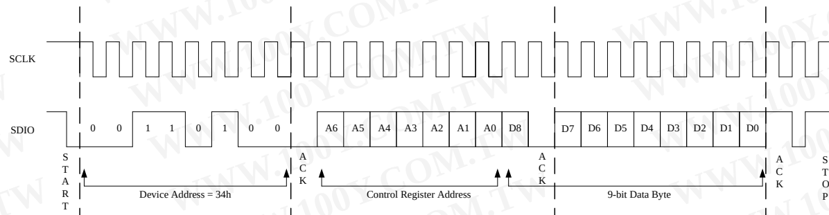
Figure 10: Byte Write Sequence
