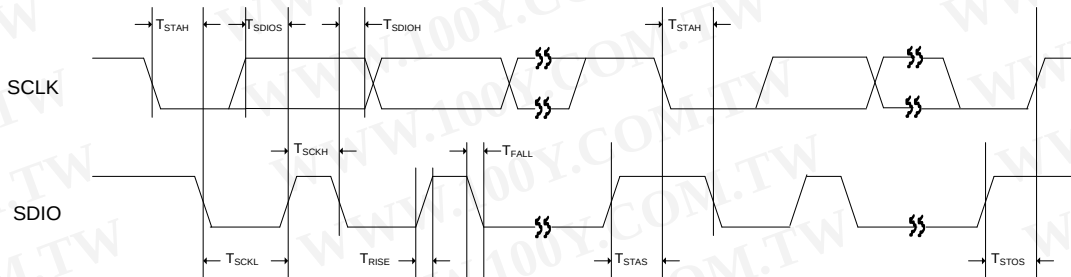
Figure 23: Two-wire Control Mode Timing
