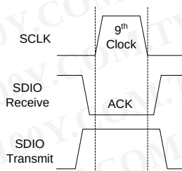
Figure 7: Valid Acknowledge
