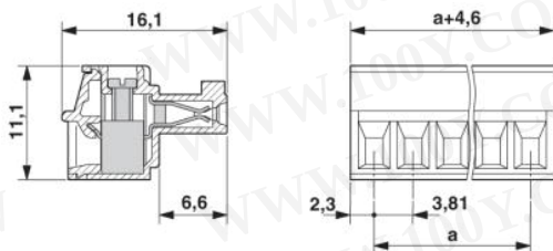
Dimensioned drawing
