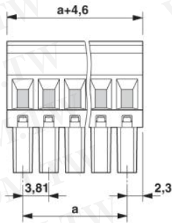
Dimensioned drawing
