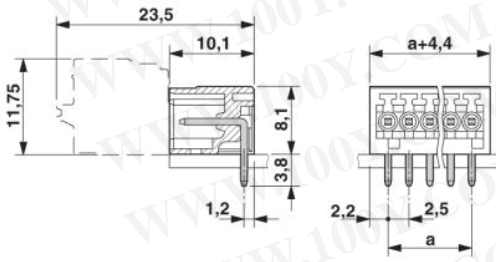
Dimensioned drawing
