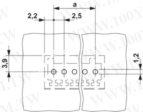
Drilling diagram
