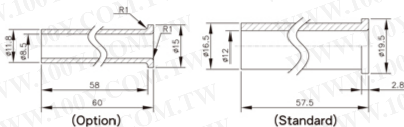
RUBBER TUBE FOR PLS-28-PM
