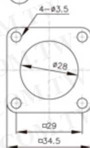
RUBBER PLATE FOR PLS-28-RF
