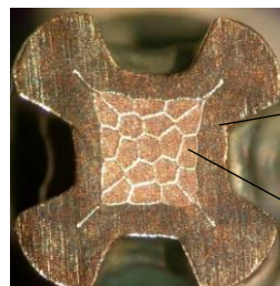
Section X-X
