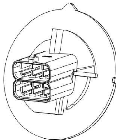
Angled Twist and Lock Cap (2x3 Shown)
