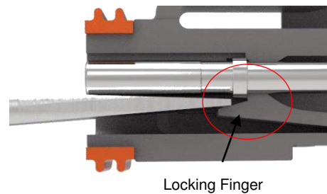
Locking Finger
