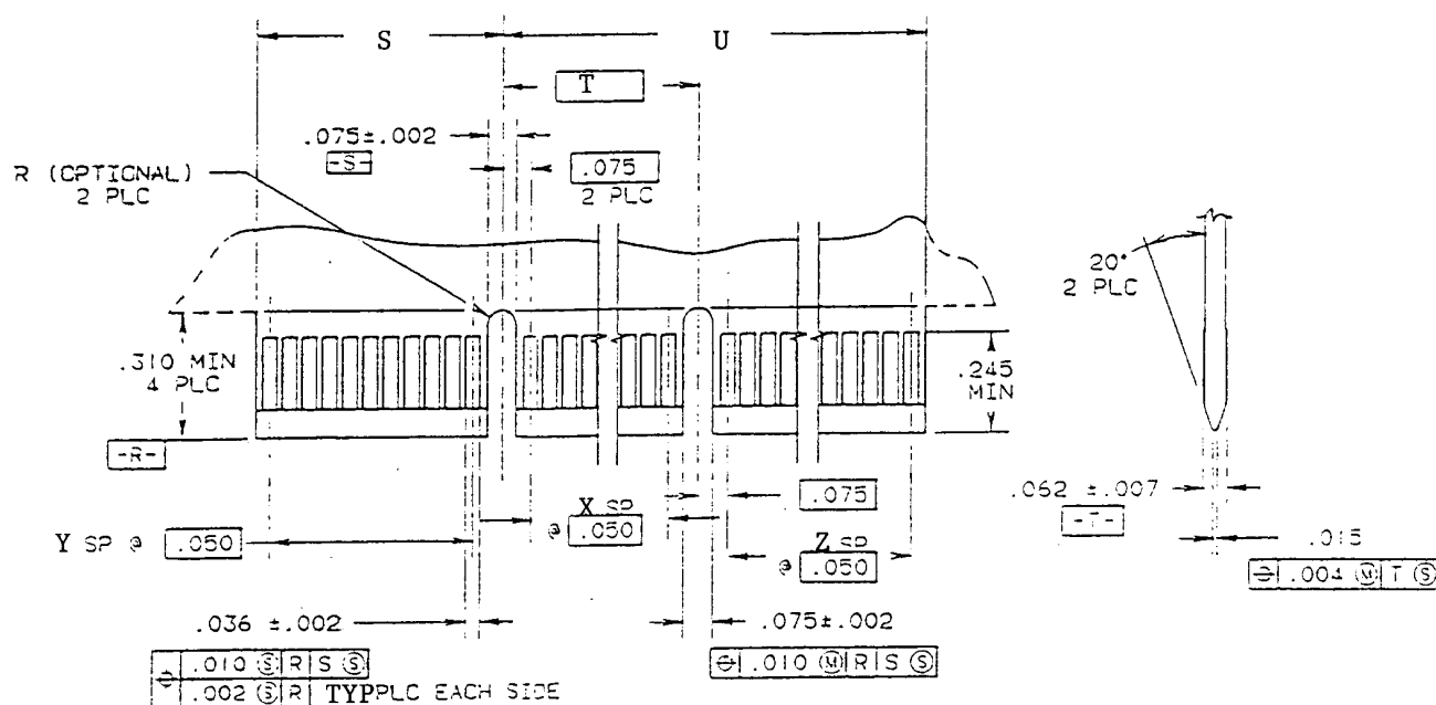
Figure 3 Test Board
