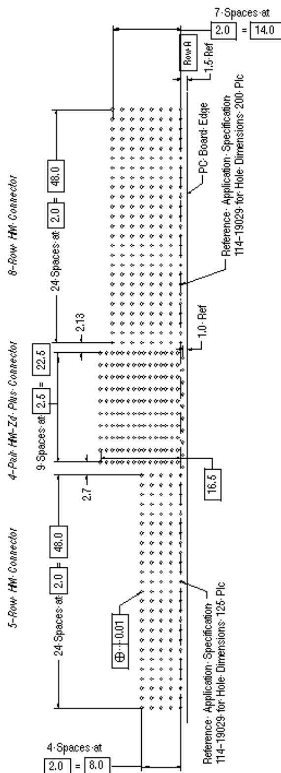
Daughter Card for -Zd-Plus-4-Pair-Connector-and-2-mm-HM-Connector-(Ref)
